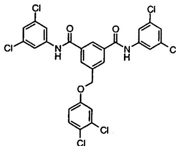
Compound # 20
